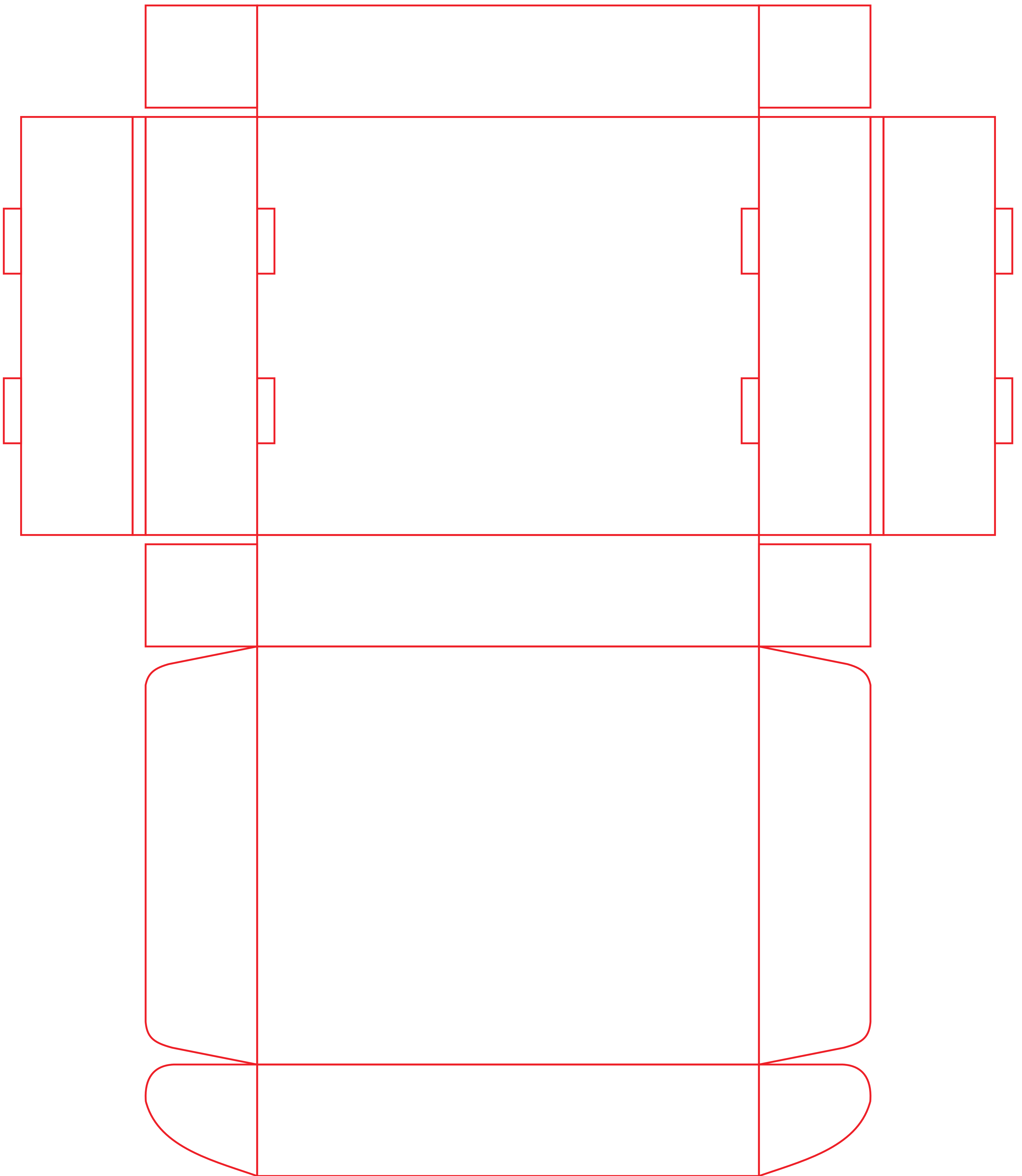
LCD2303:280x225x60mm
