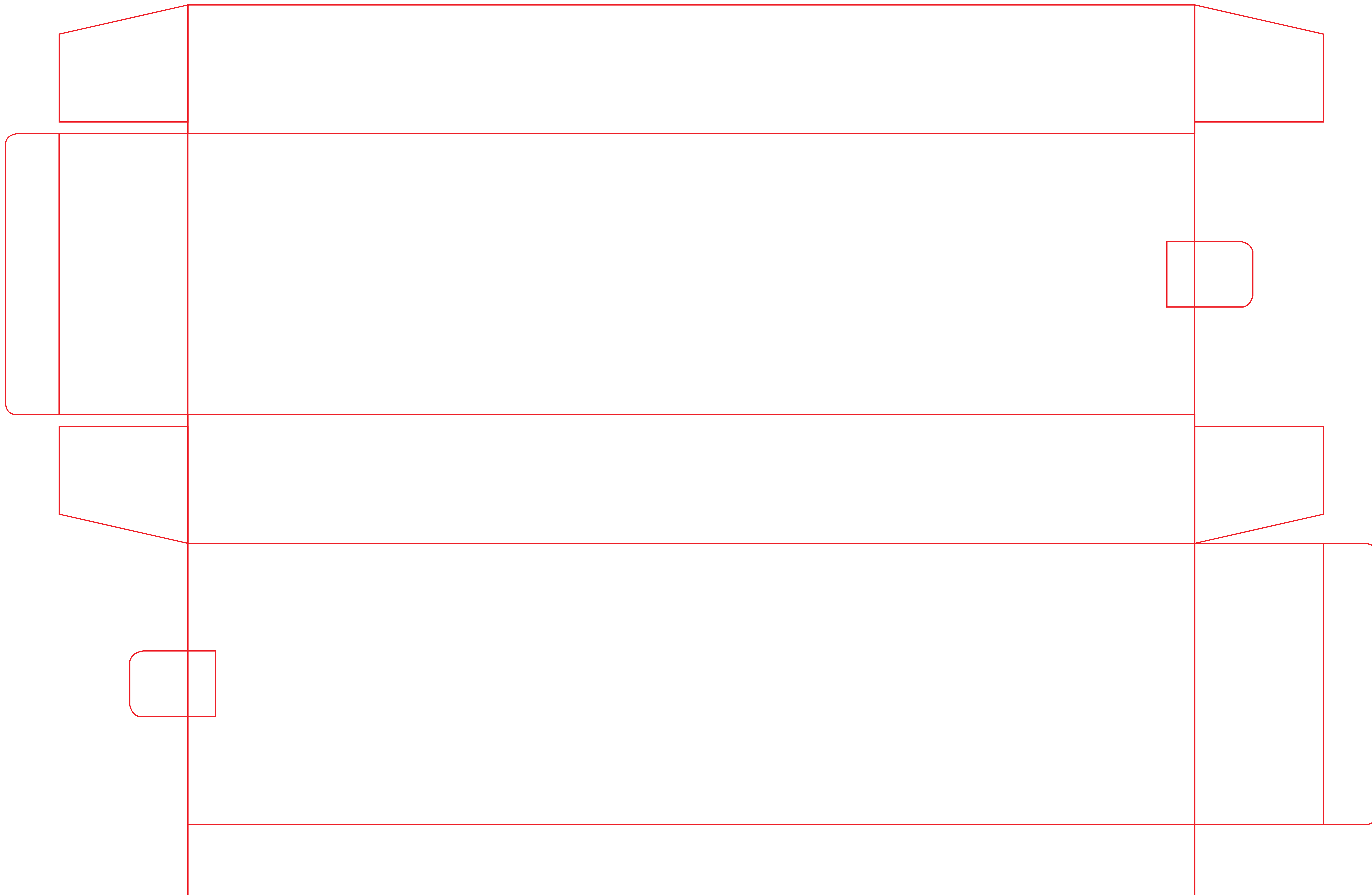
CURVE-H:860x240x110mm
